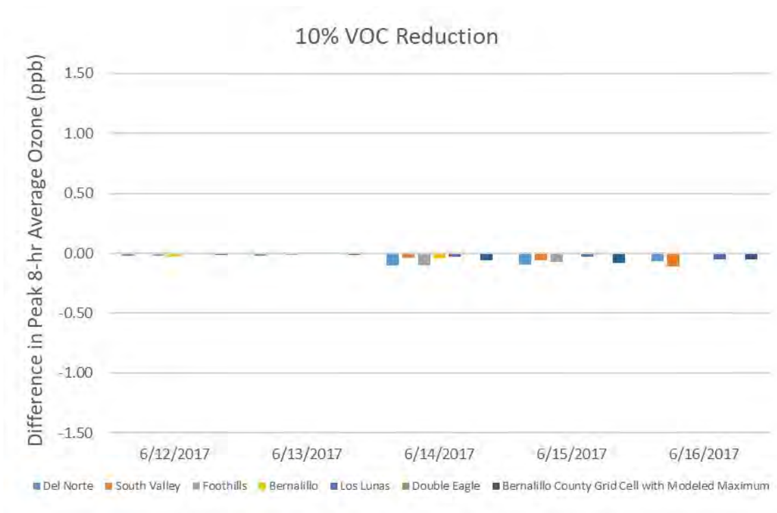
Figure 86. Differences in peak 8-hr average ozone concentrations between the 10% VOC reduction sensitivity simulation and base-case simulation in the June ozone episode at the Albuquerque MSA sites, and at the grid cell where the highest ozone concentration was modeled in the base-case simulation (Bernalillo County Grid Cell with Modeled Maximum).
