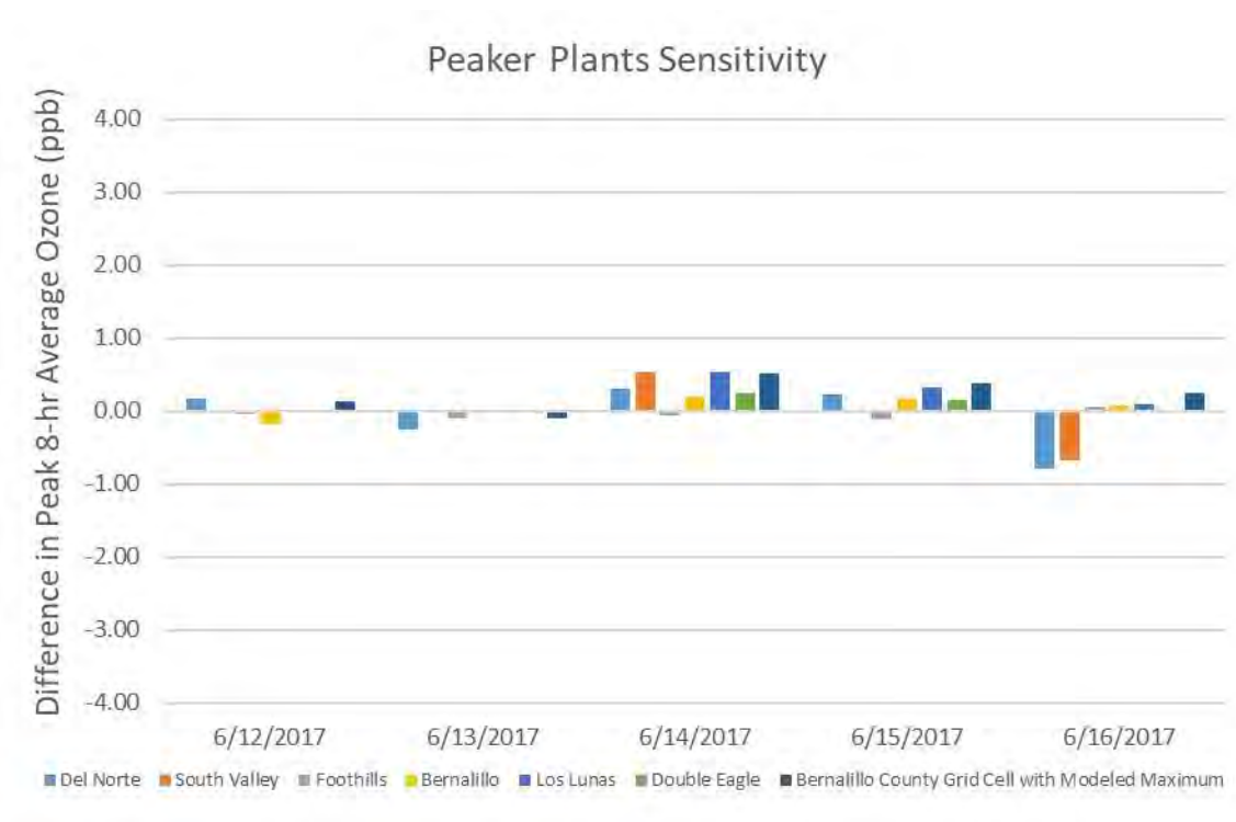
Figure 93. Differences in peak 8-hr average ozone concentrations between the simulation with Reeves and Rio Bravo power plants operating at permitted emission levels and the base-case simulation in the June ozone episode at the Albuquerque MSA sites, and at the grid cell where the highest ozone concentration was modeled in the base-case simulation (Bernalillo County Grid Cell with Modeled Maximum).
