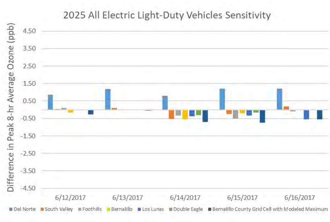
Figure 123. Differences in peak 8-hr average ozone concentrations between the 2025 all-electric light-duty vehicles sensitivity simulation and the 2025 base-case simulation in the regionally dominated ozone episode at the Albuquerque MSA sites, and at the grid cell where the highest ozone concentration was modeled in the base-case simulation (Bernalillo County Grid Cell with Modeled Maximum).
