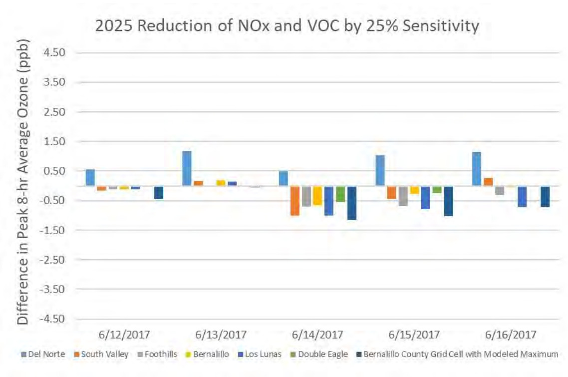
Figure 120. Differences in peak 8-hr average ozone concentrations between the 2025 anthropogenic NO x and VOC 25% reduction sensitivity simulation and the 2025 base-case simulation in the regionally dominated ozone episode at the Albuquerque MSA sites, and at the grid cell where the highest ozone concentration was modeled in the base-case simulation (Bernalillo County Grid Cell with Modeled Maximum).
