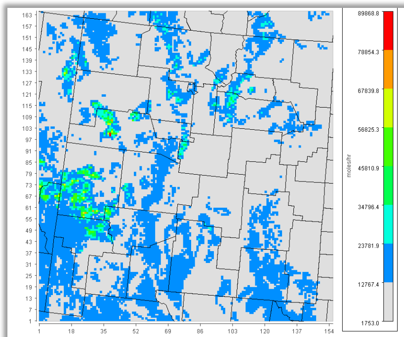
Figure 50. Biogenic VOC emissions on July 7, 2017 for the 4-km domain.
