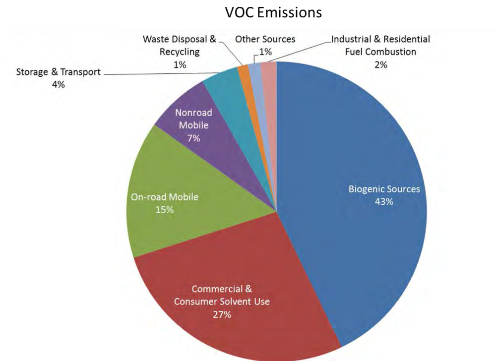
Figure 26. Annual 2014 VOC emissions in Albuquerque/Bernalillo County.
