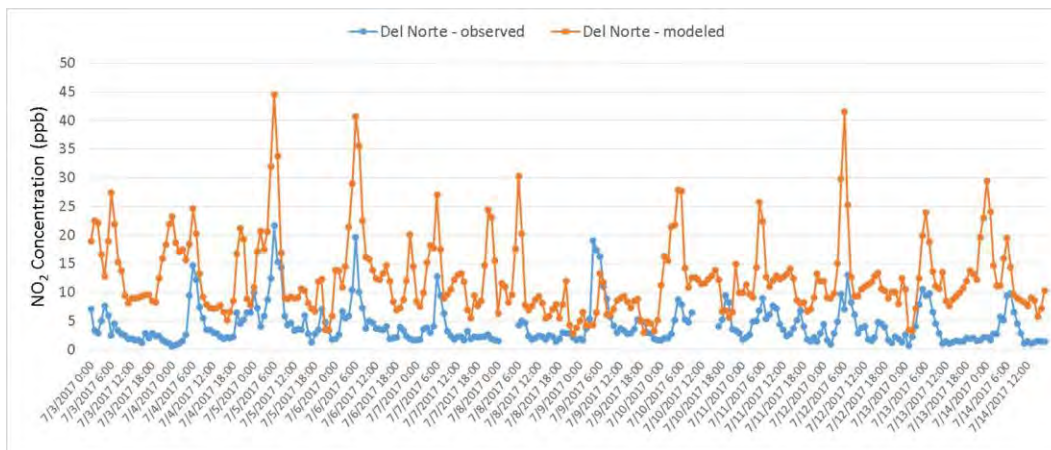
Figure 70. Hourly observed (blue line) and modeled (red line) NO 2 concentrations at the Del Norte monitor during the July episode.
