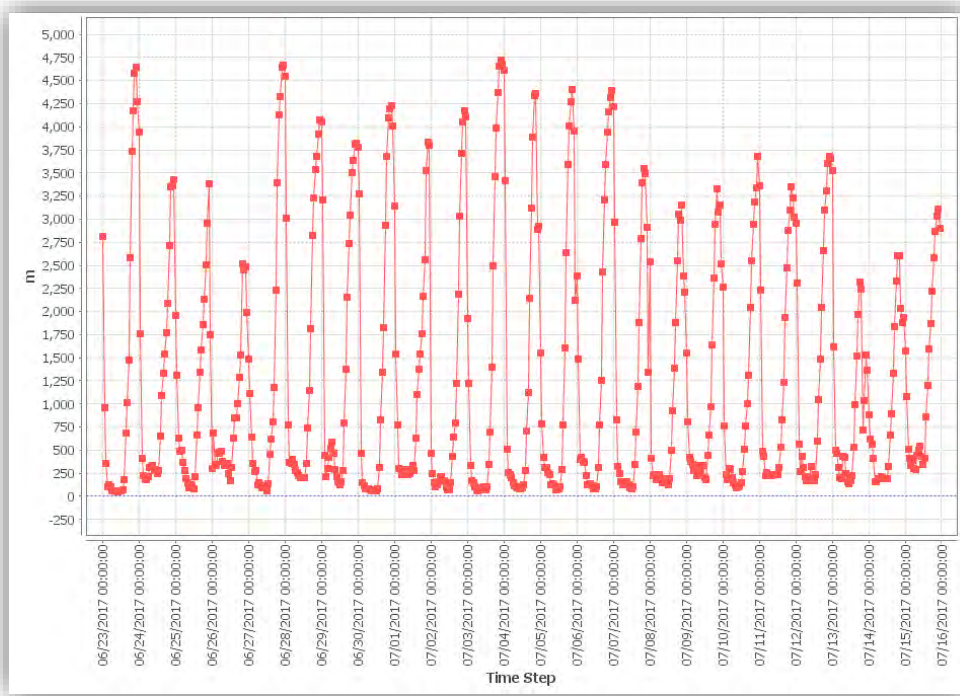
Figure 44. WRF boundary layer heights (meters above ground level) during the July modeling episode at Albuquerque. Times are in UTC.
